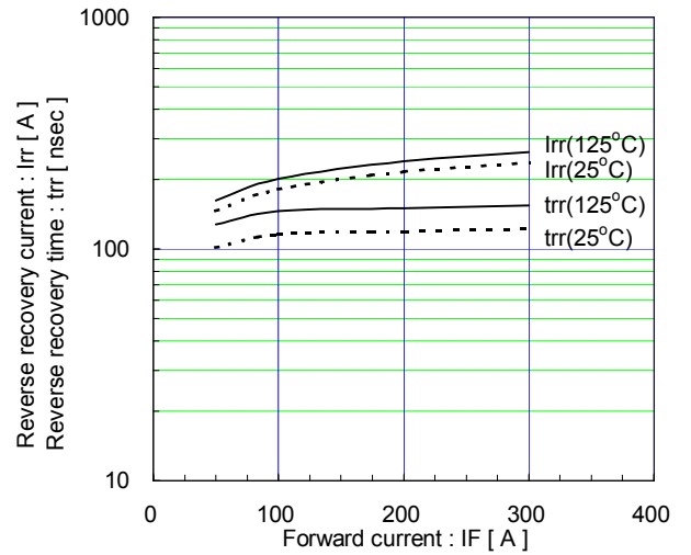
Reverse recovery characteristics (typ.) Vcc=600V, VGE=±15V, RG=3.0Ω
